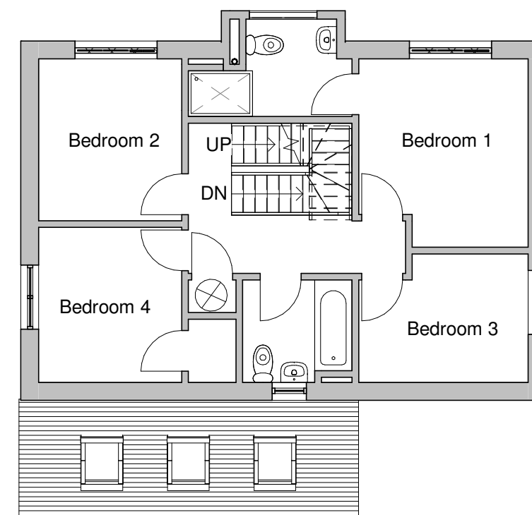
Proposed First Floor 1 : 100
