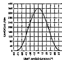
SYMMETRIC REFLECTOR UM70S 70W E27
