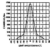
CIRCULAR PROJECTOR UMP70 70W RX7S
