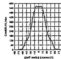
SYMMETRIC REFLECTOR UM150MHL 150W RX7S
