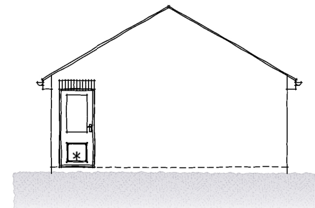
SIDE ELEVATION * DOOR TO PLOT 110 ONLY
