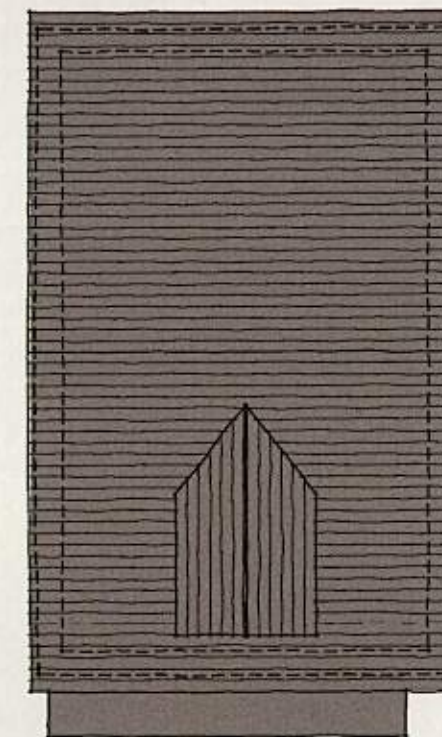
ROOF PLAN
