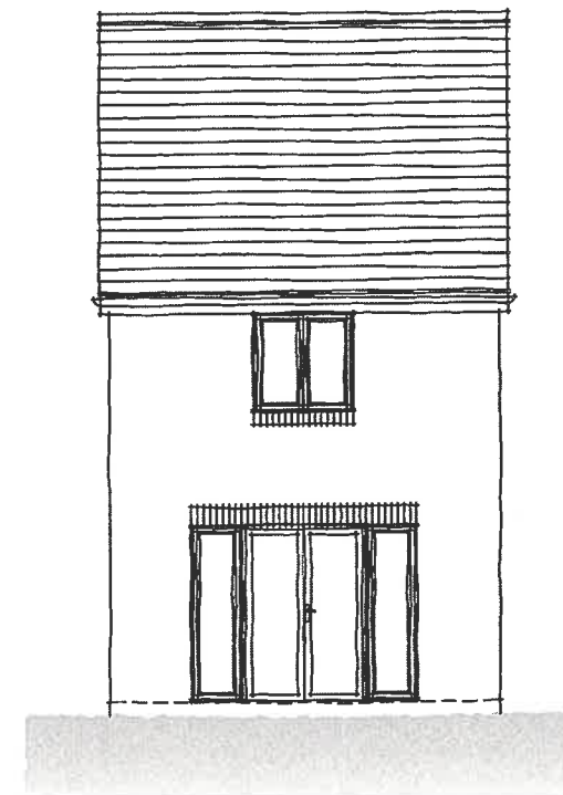
REAR ELEVATION
