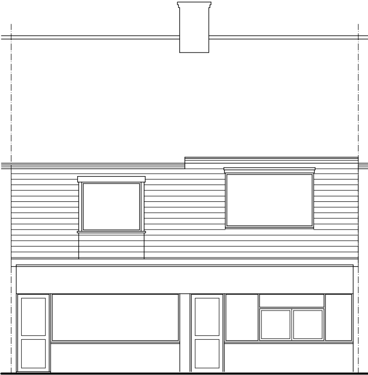
Front Elevation
