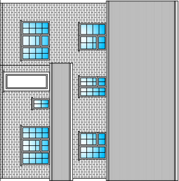
EXISTING SOUTH ELEVATION 1:100
