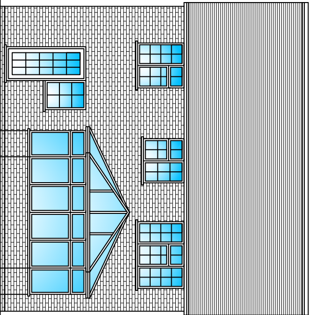
EXISTING NORTH ELEVATION 1:100
