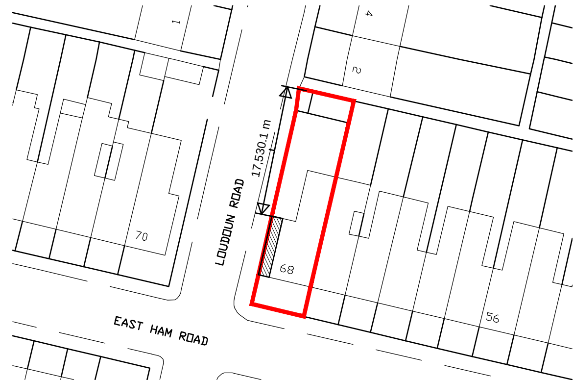
BLOCK PLAN(1:500)
