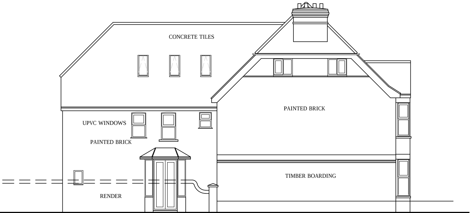
LOUDOUN ROAD ELEVATION
