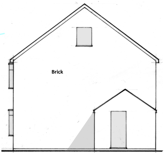
Existing Side Elevation (South) 1:100
