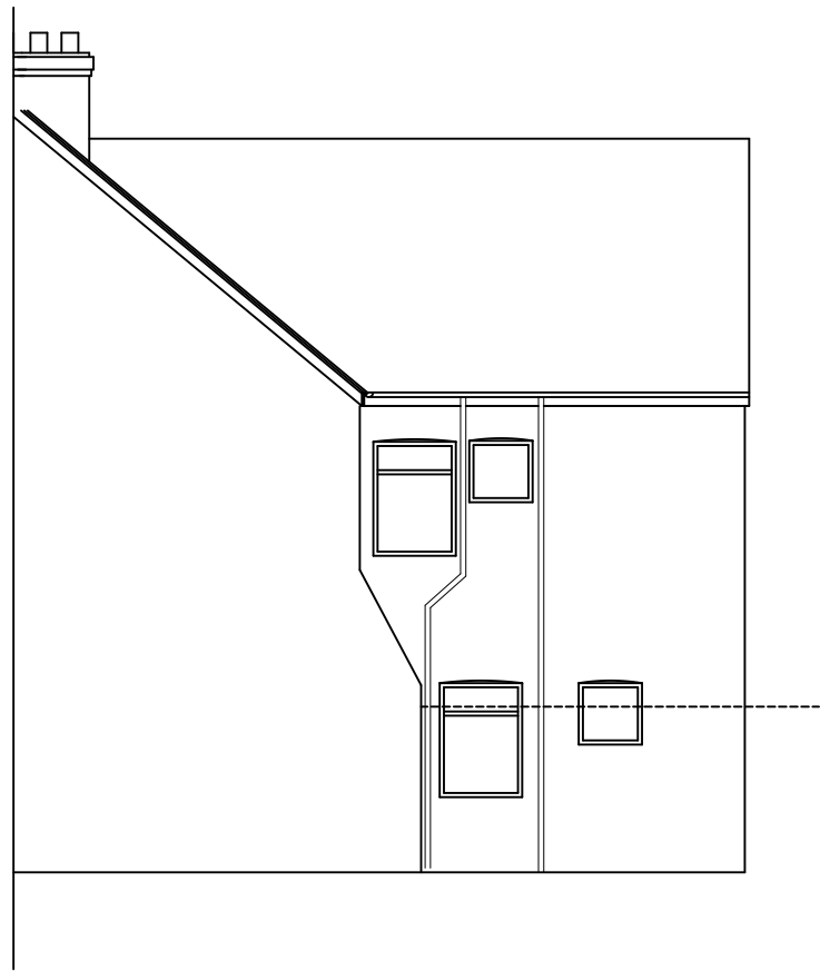
EXISTING SOUTH ELEVATION
