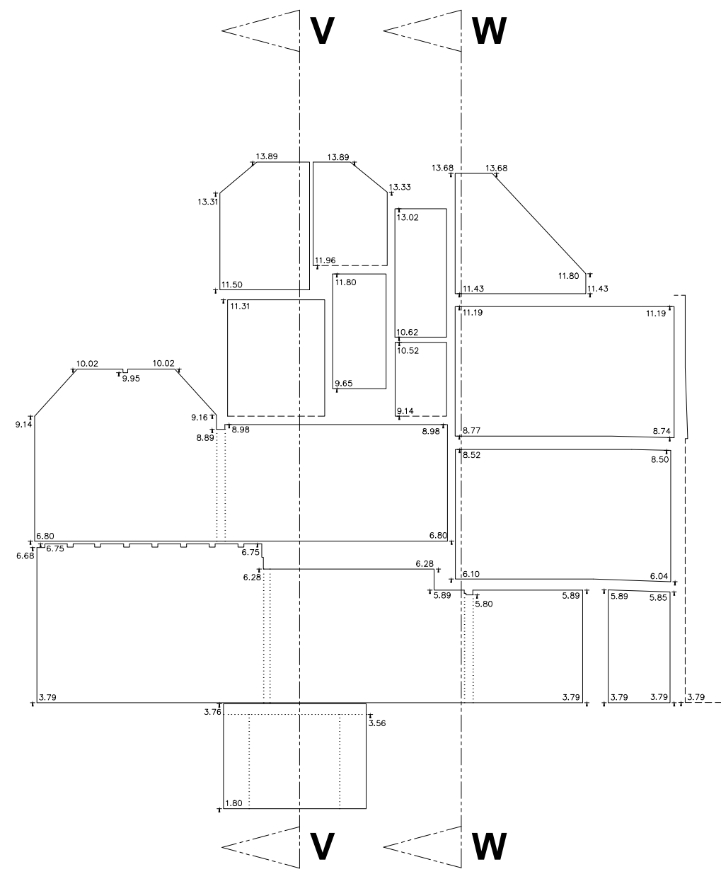
SECTION U-U
