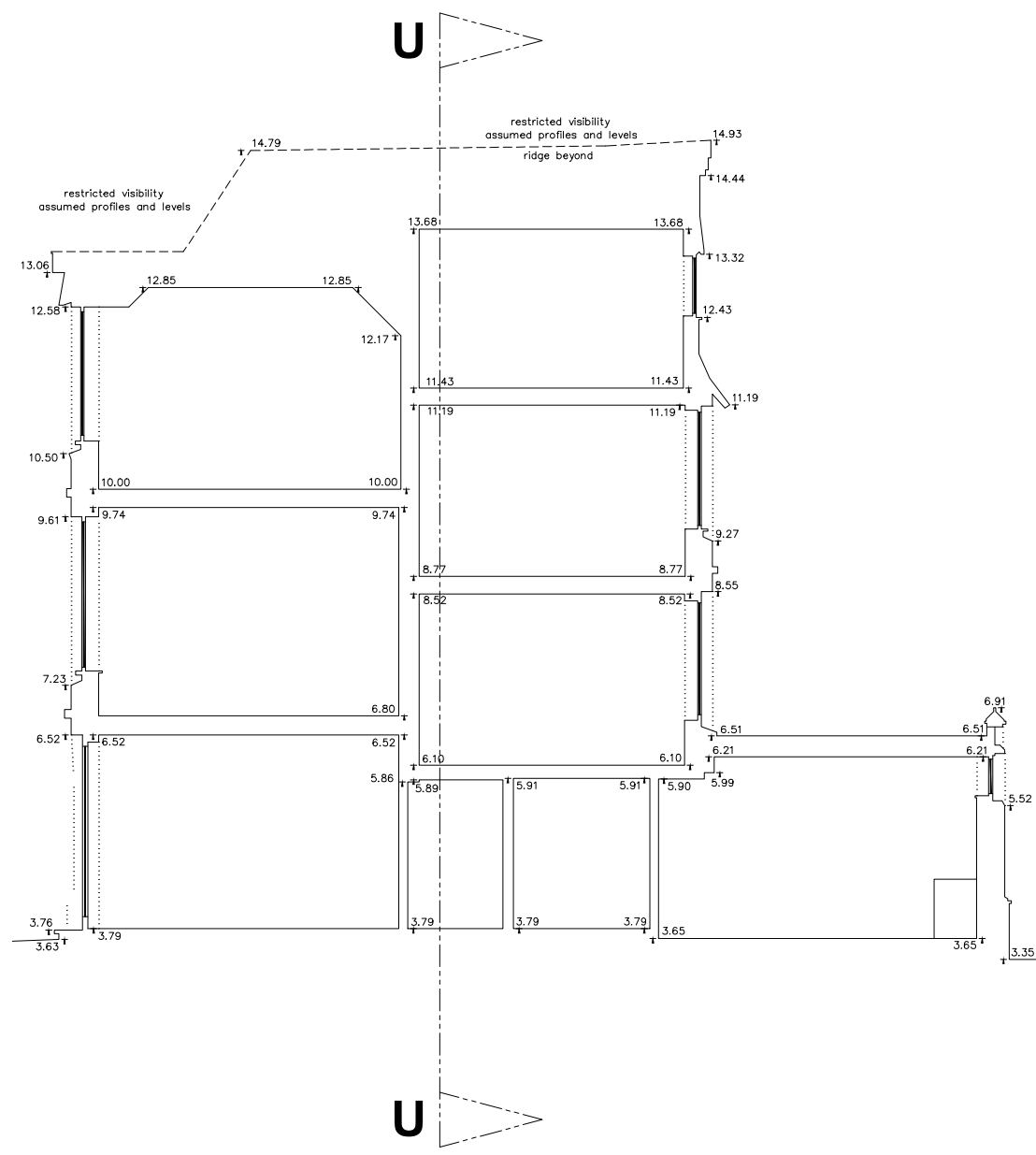
SECTION W-W
