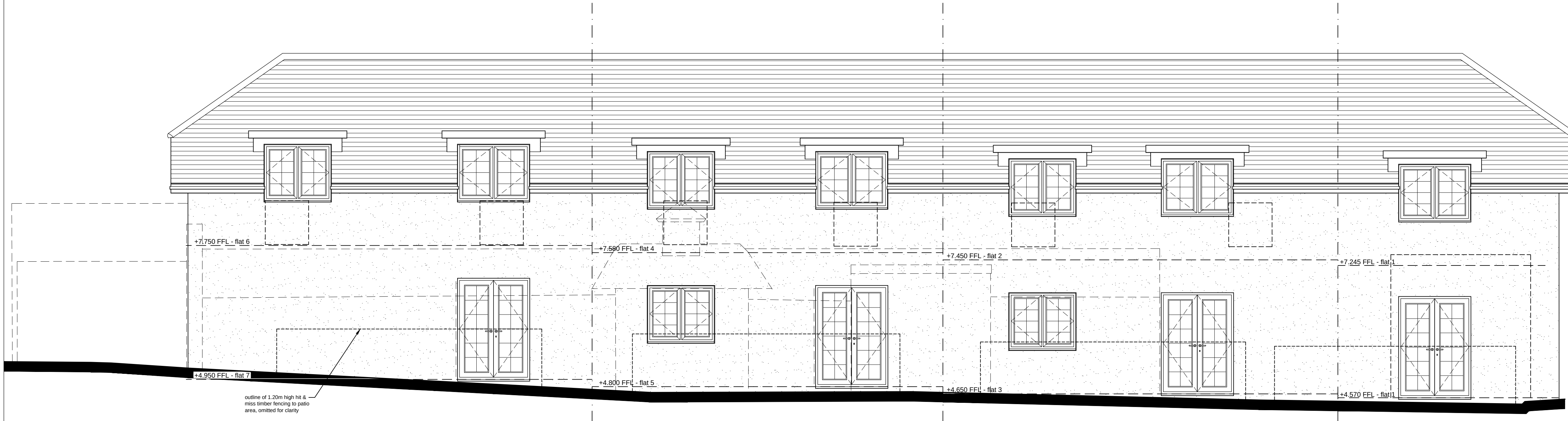
Western Elevation As Proposed to Flats 1 - 7 - 1:50 @ A1
