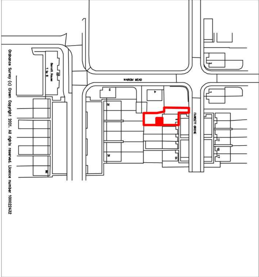
Location PLAN 1:1250
