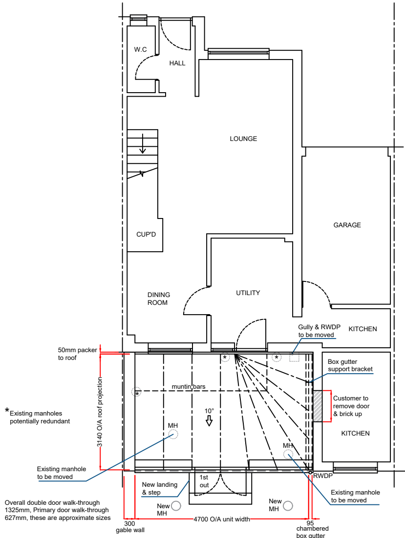
PLAN
