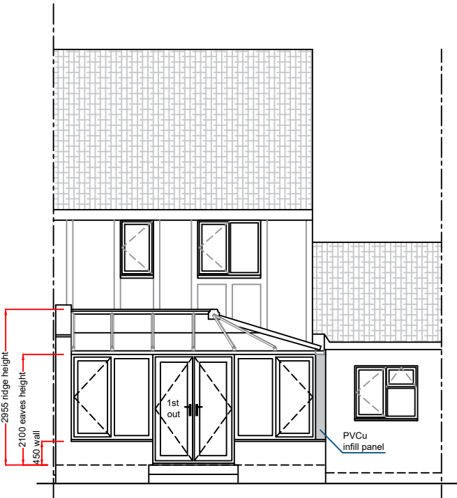
REAR ELEVATION
