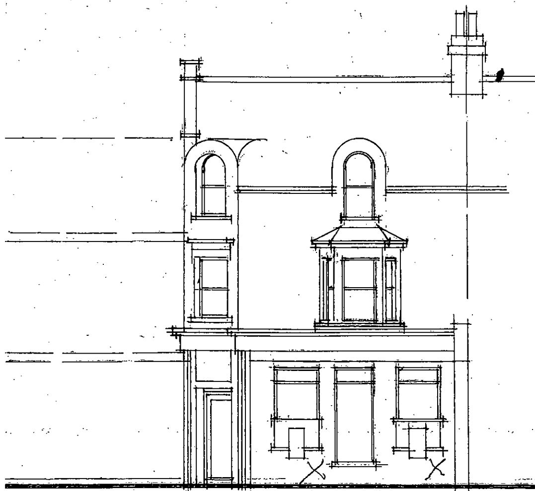
NORTH ELEVATION
