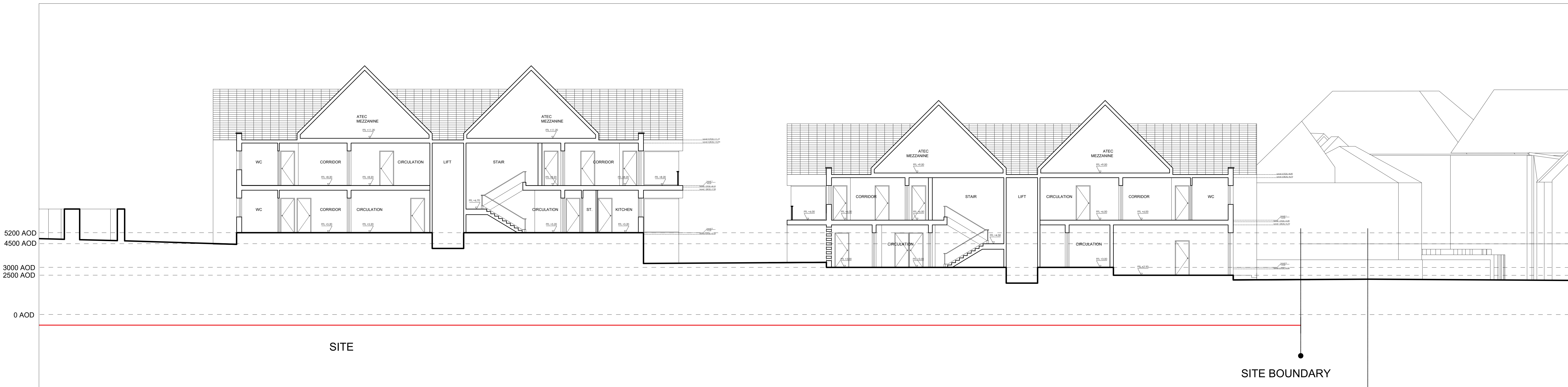
Section D-D Scale 1:100 @ A0
