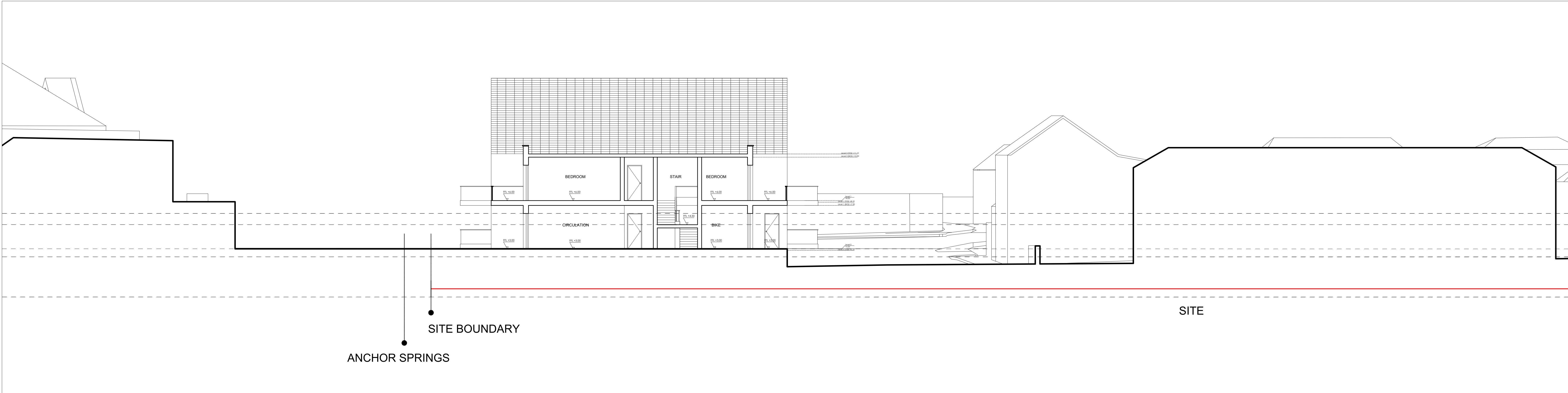
Section A-A Scale 1:100 @ A0
