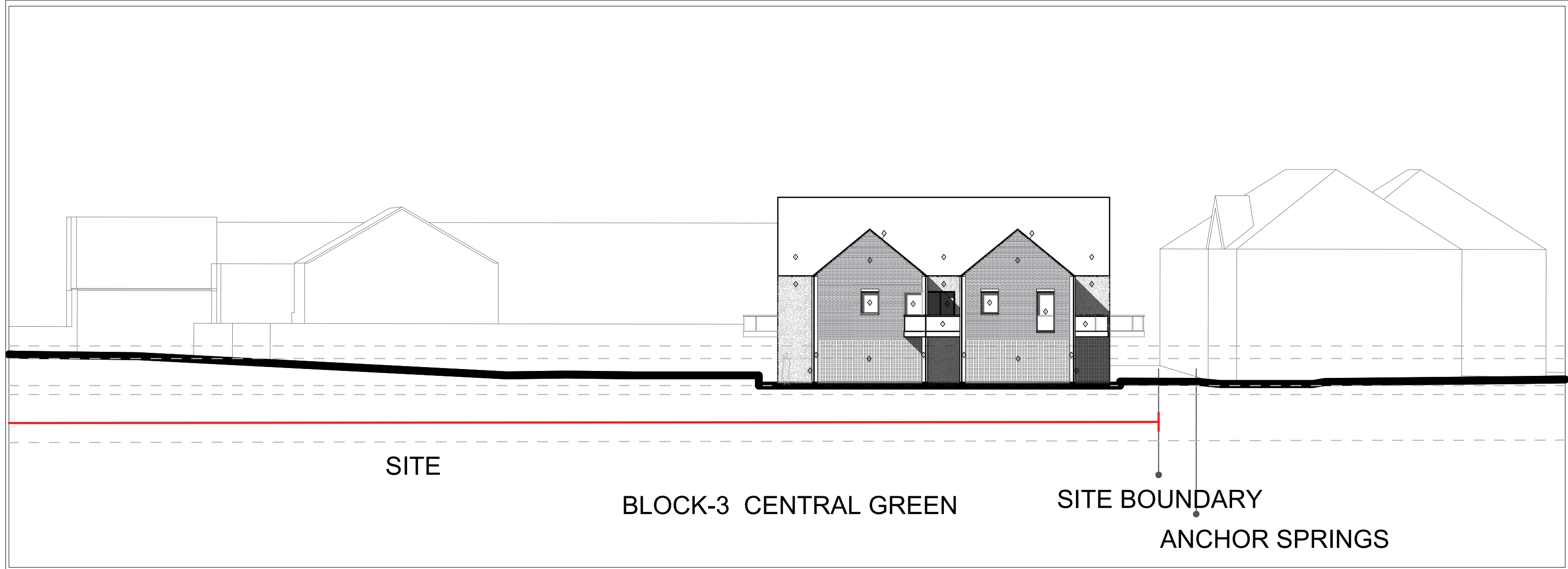
Elevation D 1:100 @ A0
