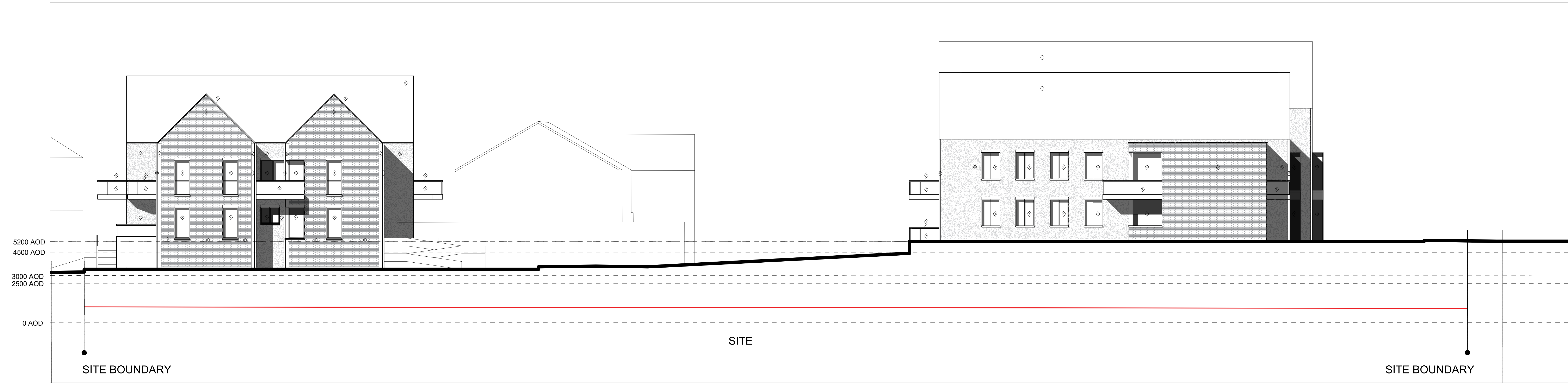
Elevation C 1:100 @ A0
