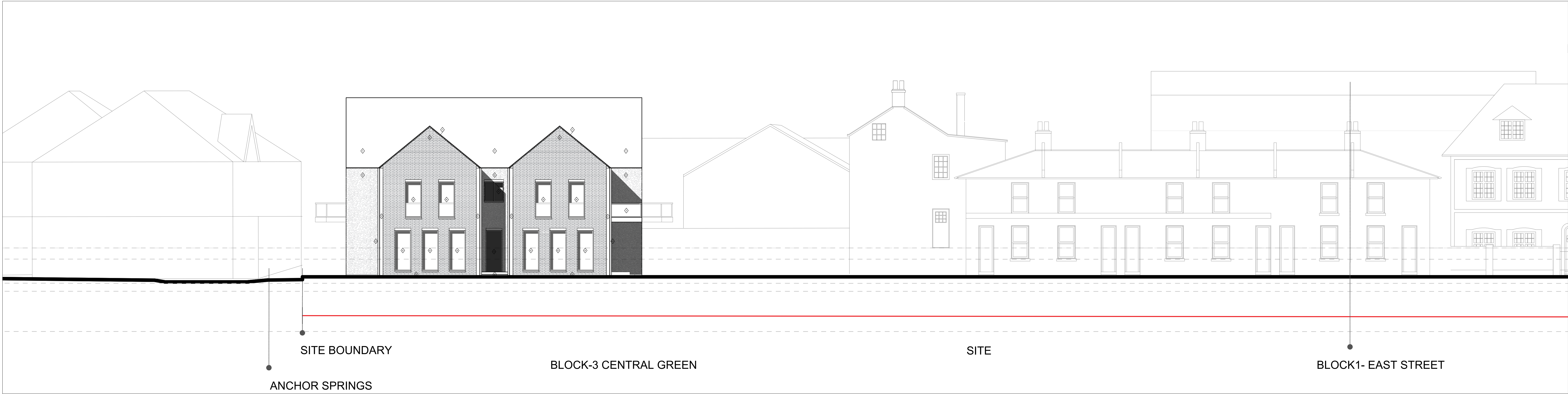
Elevation G | East Street Scale 1:100 @ A0
