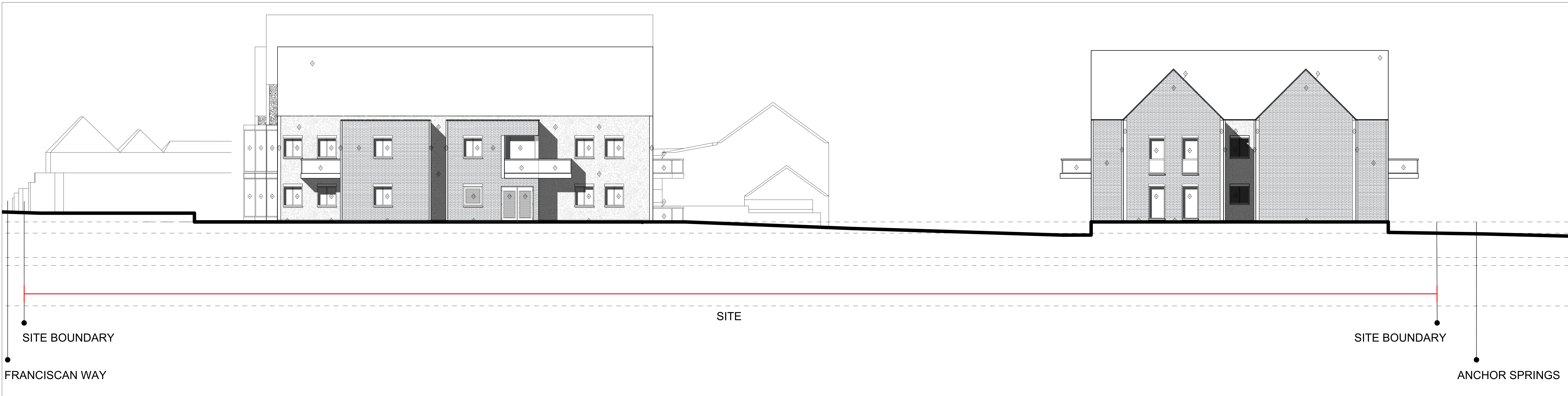
0 4 8 12 16 20 Elevation H 1:100 @ A0
