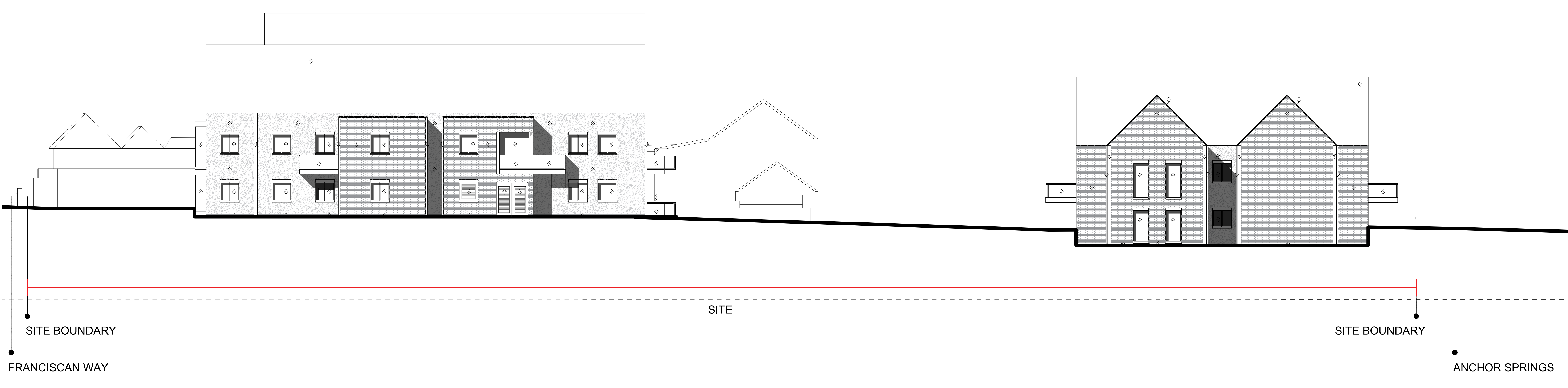
0 4 8 12 16 20 Elevation H 1:100 @ A0
