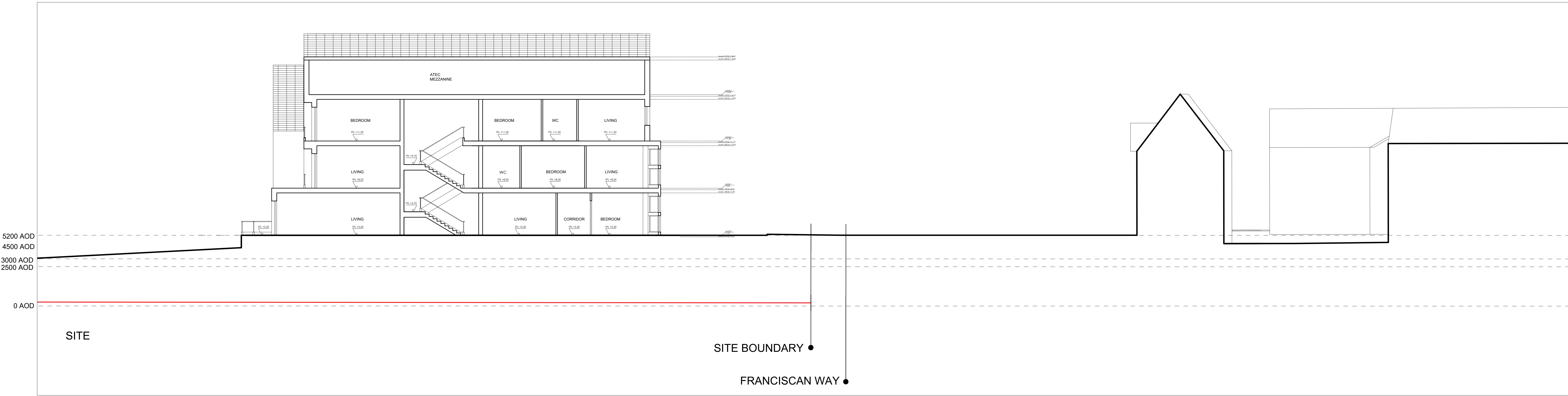
Section C-C Scale 1:100 @ A0
