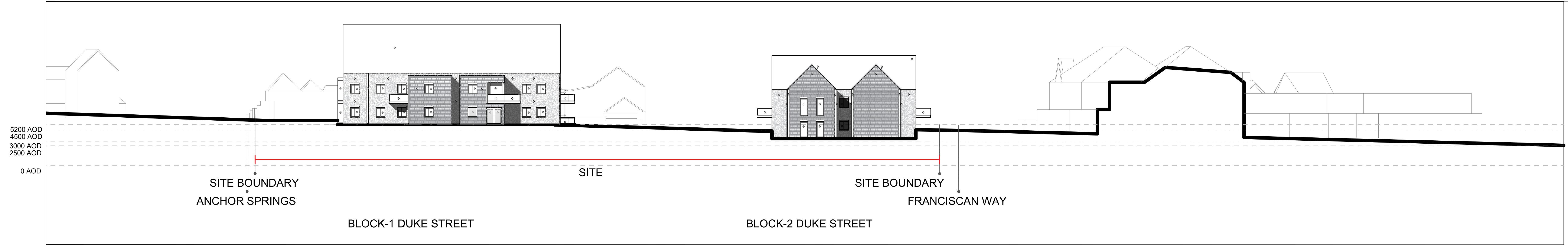
Elevation H 1:100 @ A0
