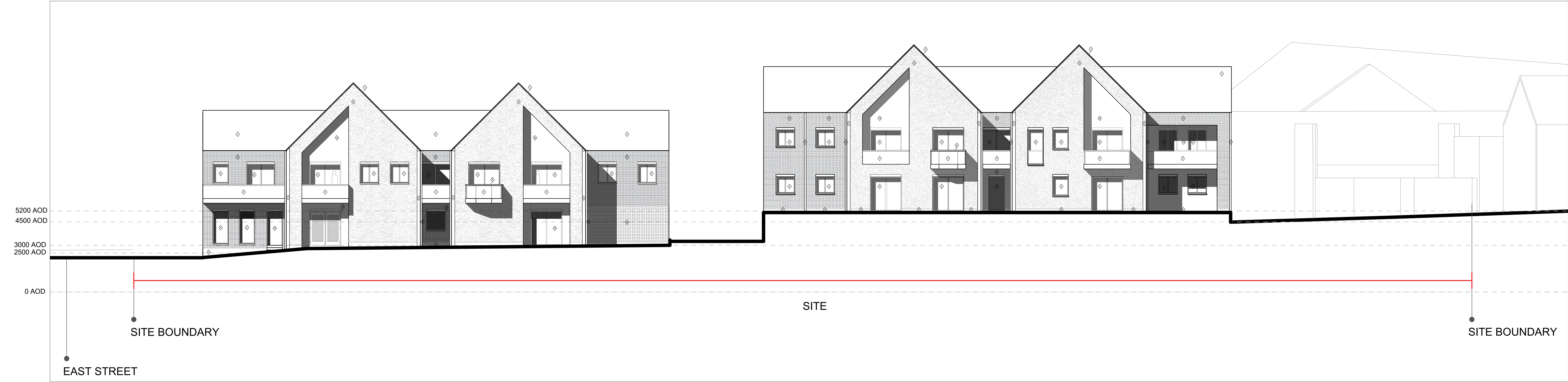
Elevation E | Avon Road Scale 1:100 @ A0
