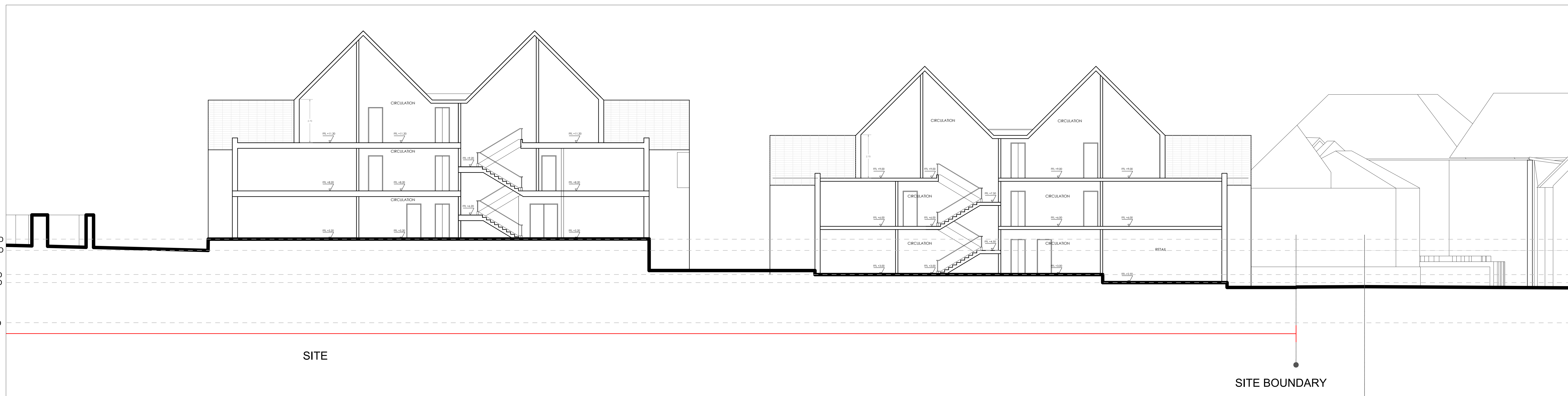
0 4 8 12 16 20 Section D-D Scale 1:100 @ A0
