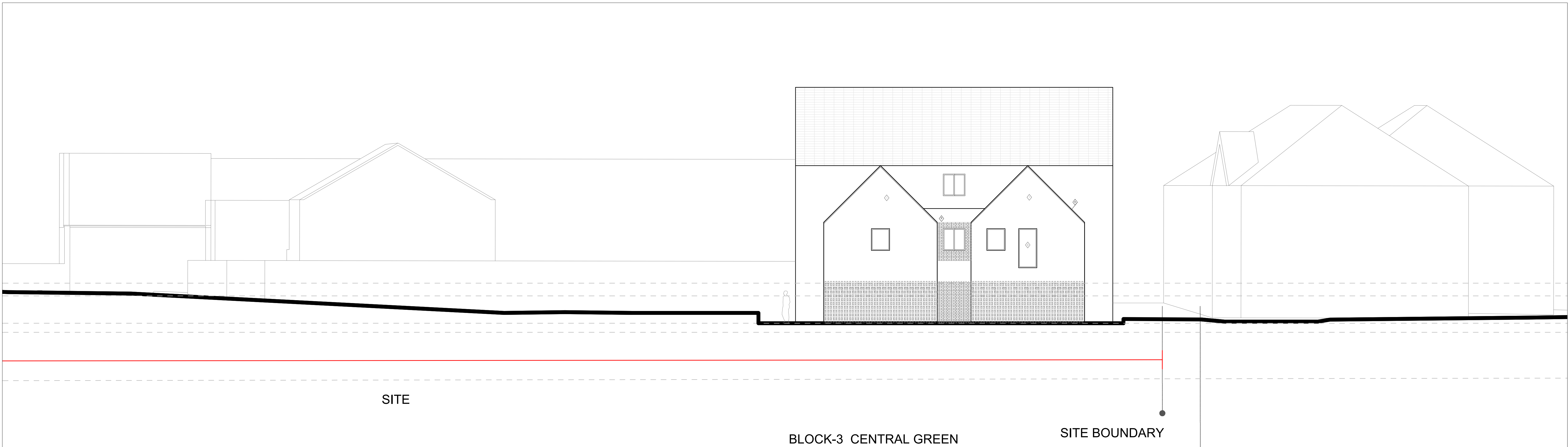
Elevation D Scale 1:100 @ A0
