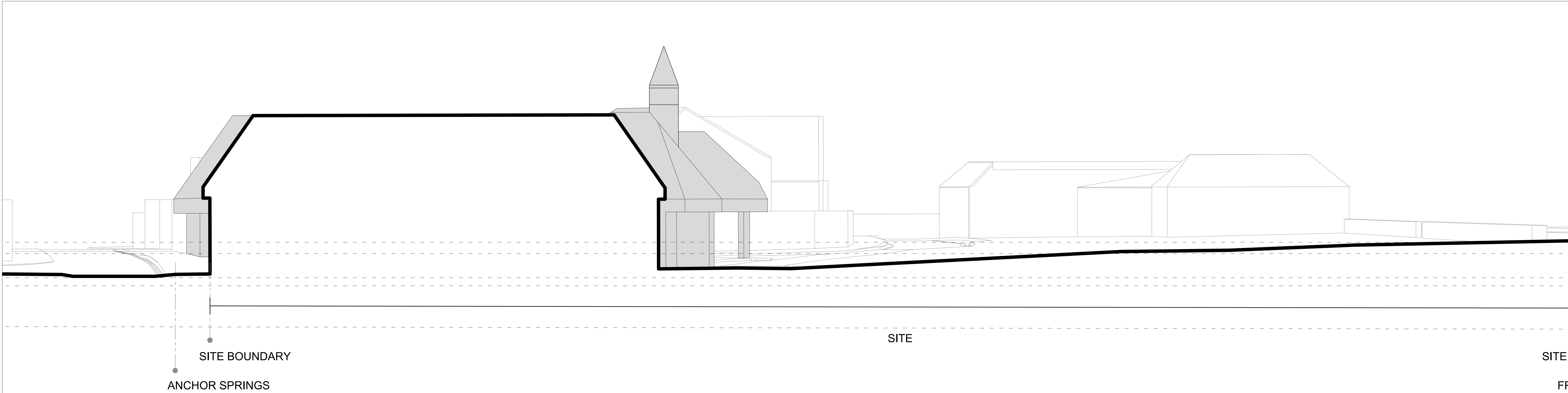
0 4 8 12 16 20 Section C-C Scale 1:100 @ A0
