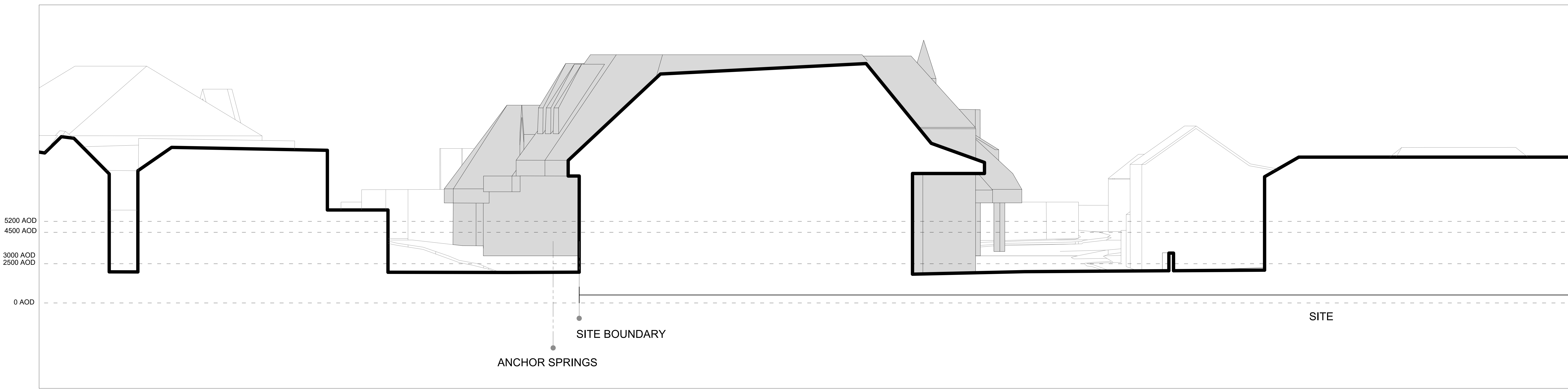
Section A-A Scale 1:100 @ A0
