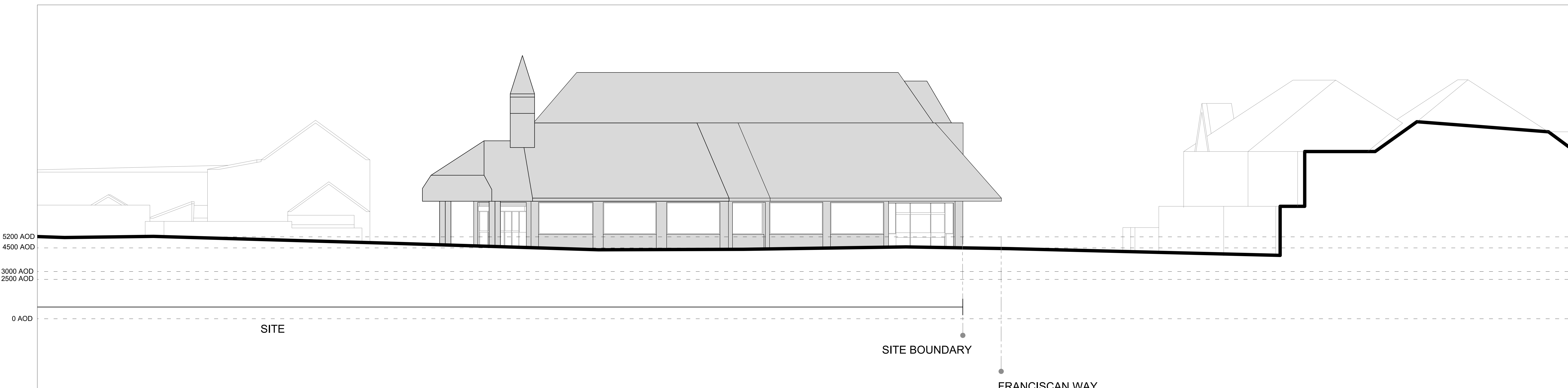
Elevation H | Duke Street Scale 1:100 @ A0
