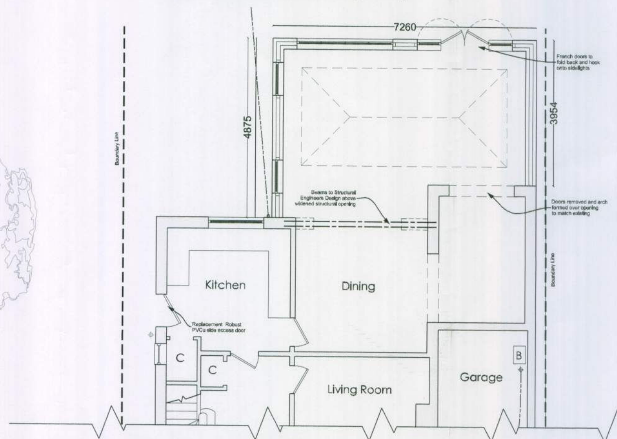
Proposed Part Floor Plan (1:100)
