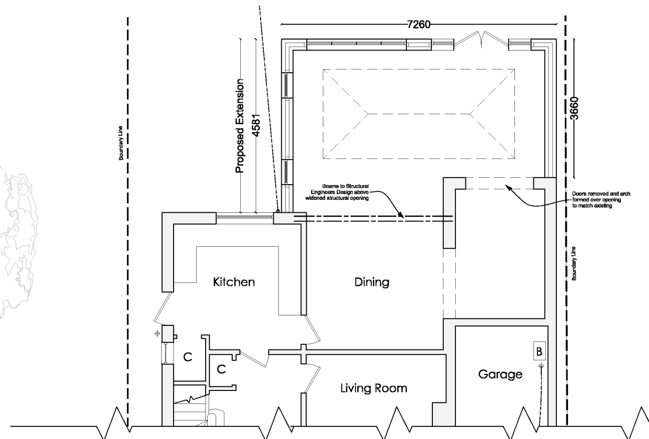
Proposed Part Floor Plan (1:100)
