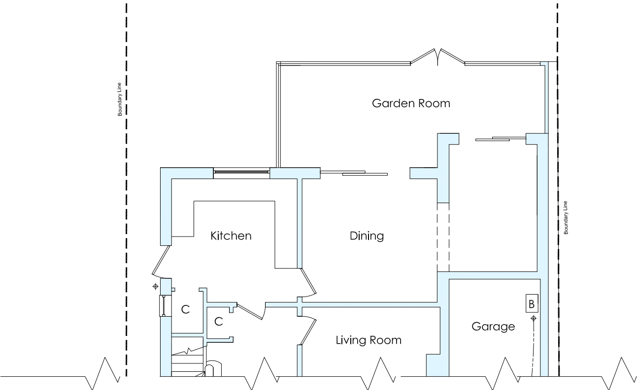
Existing Part Floor Plan (1:100)
