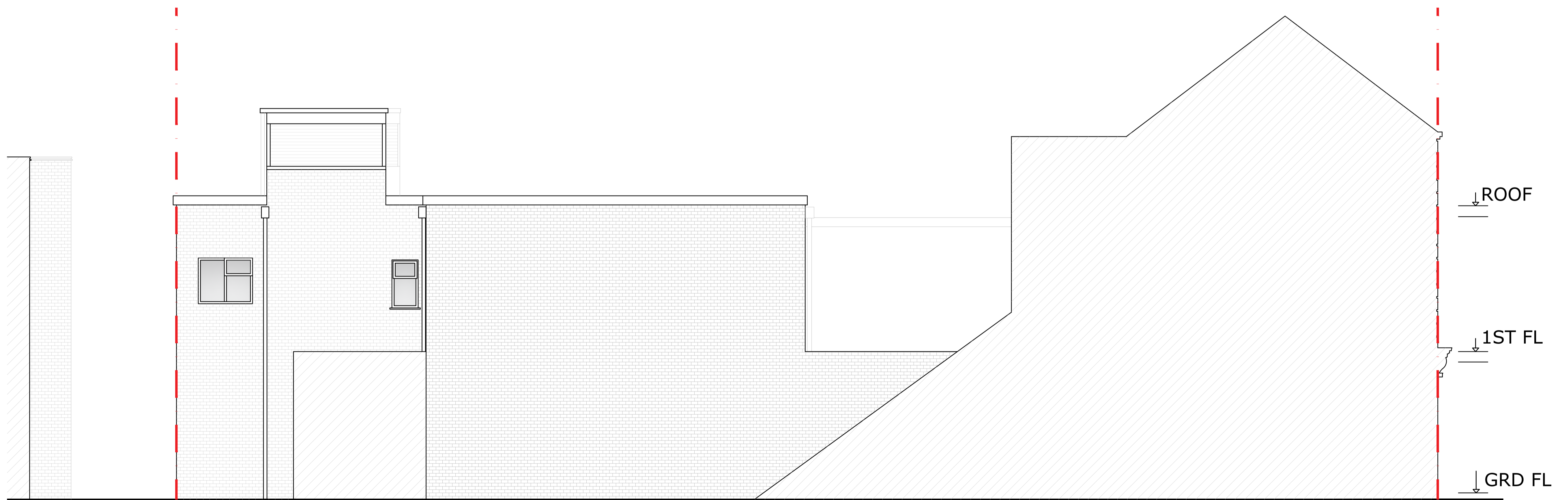
PROPOSED SIDE ELEVATION 2
