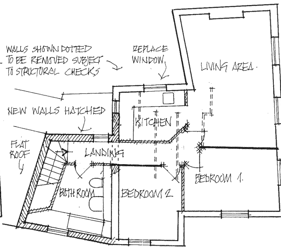
FLAT 2 / SECOND FLOOR
