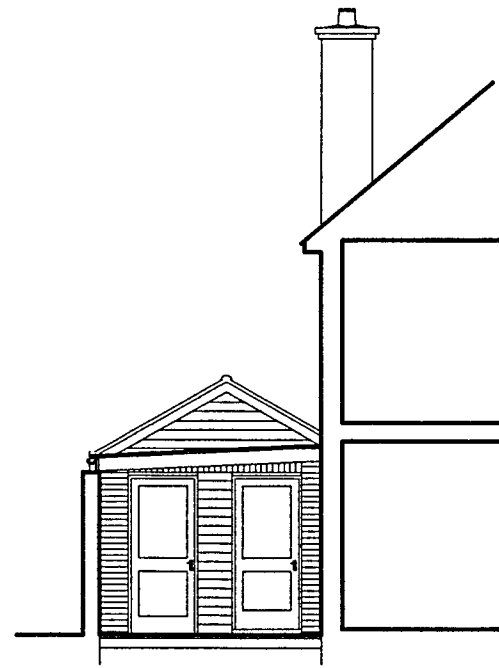
Utility Room West Elevation to Car Port:
