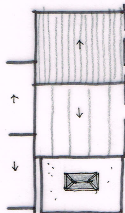
ROOF PLAN 1:200
