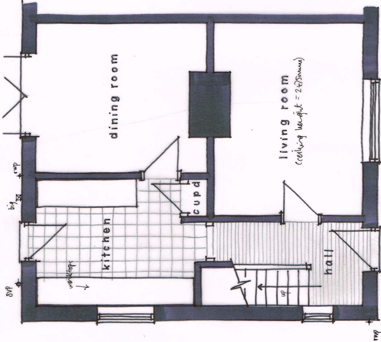
GROUND FLOOR PLAN 1:50 @ A3
