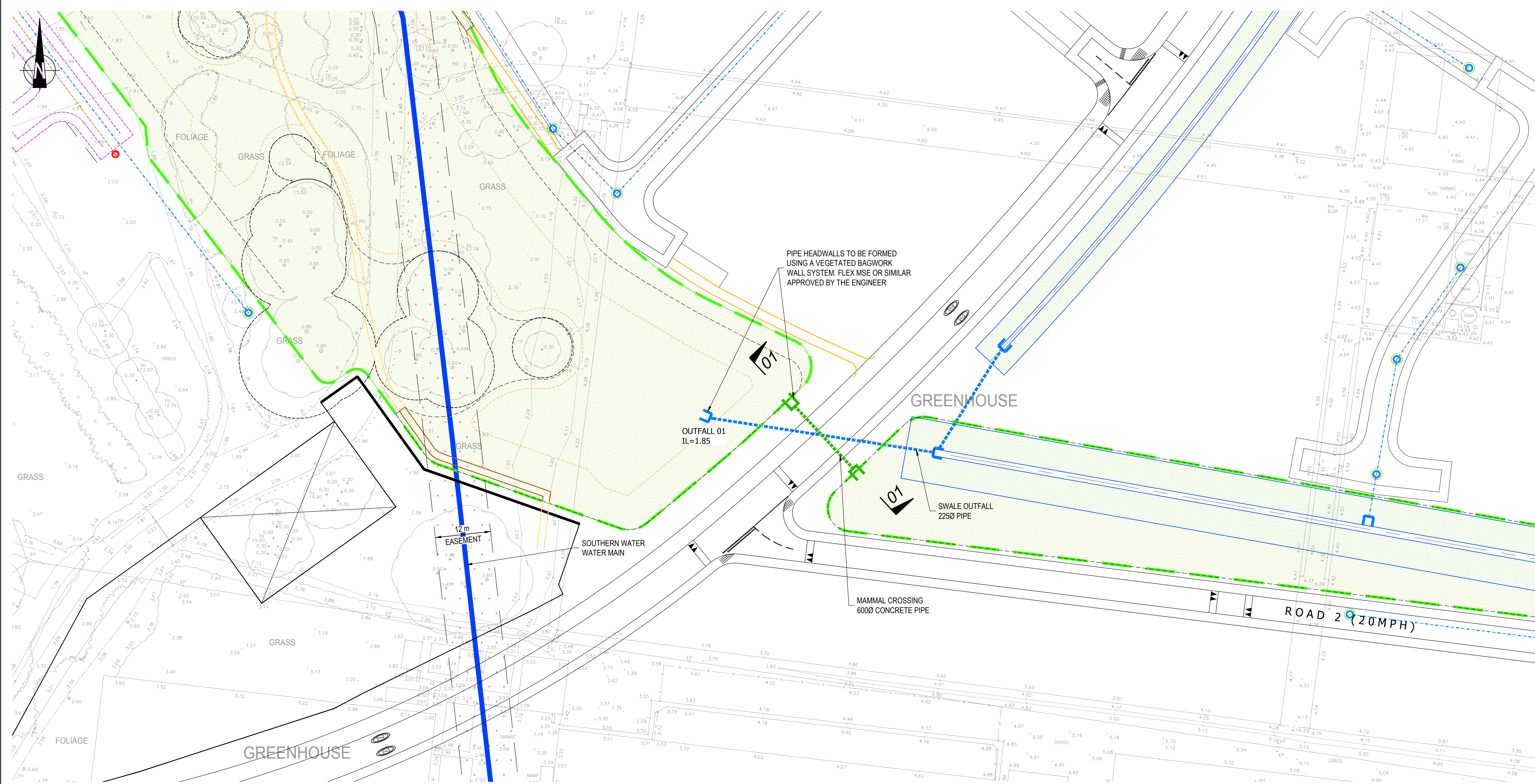
PLAN 1:500
