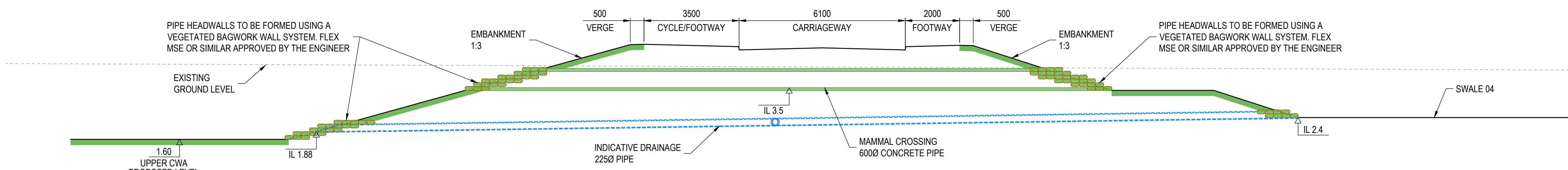
SECTION 01-01 (OUTFALL PIPE SHOWN RELATIVE TO MAMMAL CROSSING) 1:100
