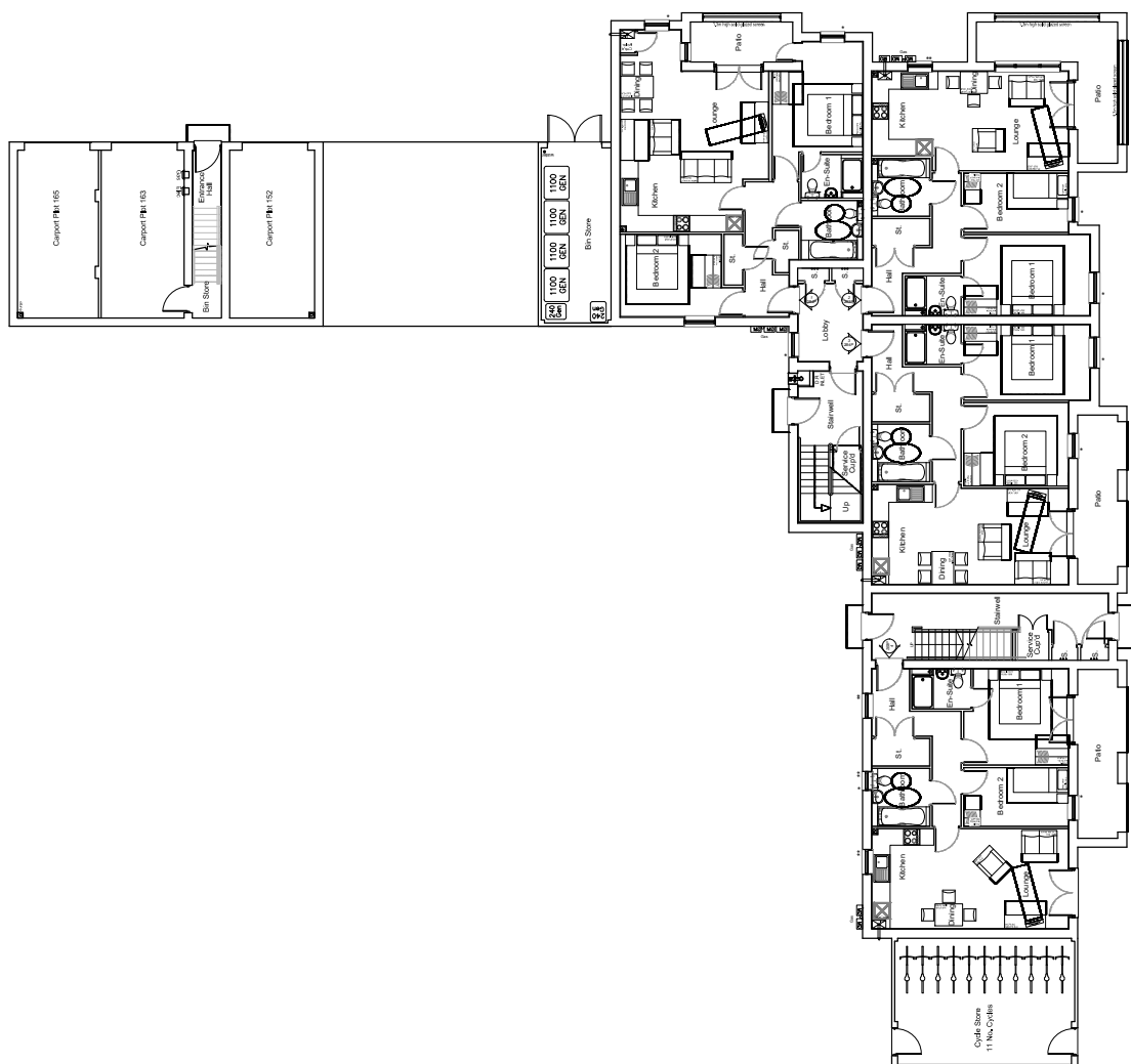
Ground Floor Plan ** - False Panel * - Obscured Glazing
