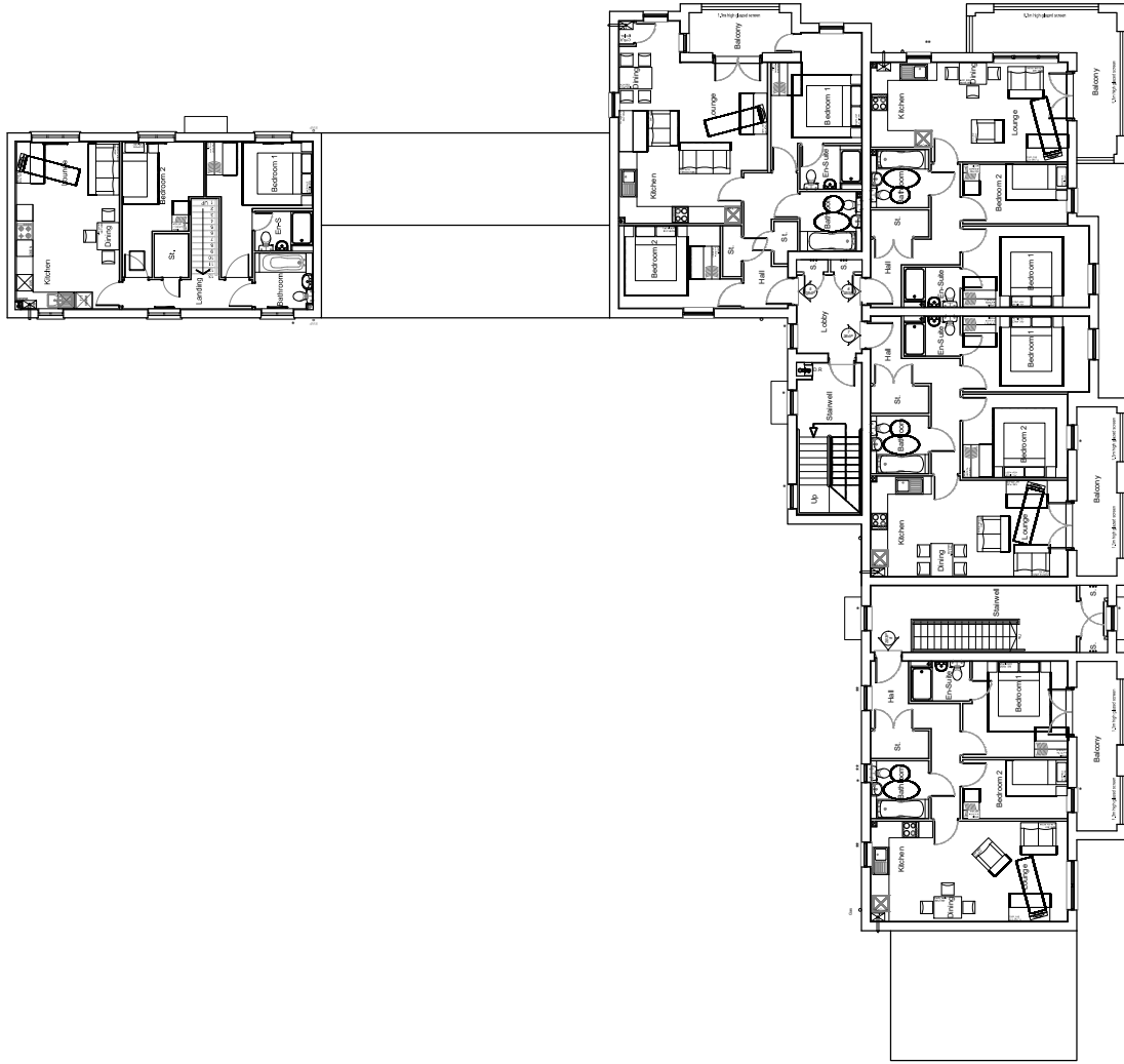
First Floor Plan ** - False Panel * - Obscured Glazing
