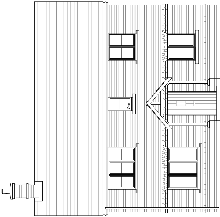
Front Elevation Obs - Obscured Glazing
