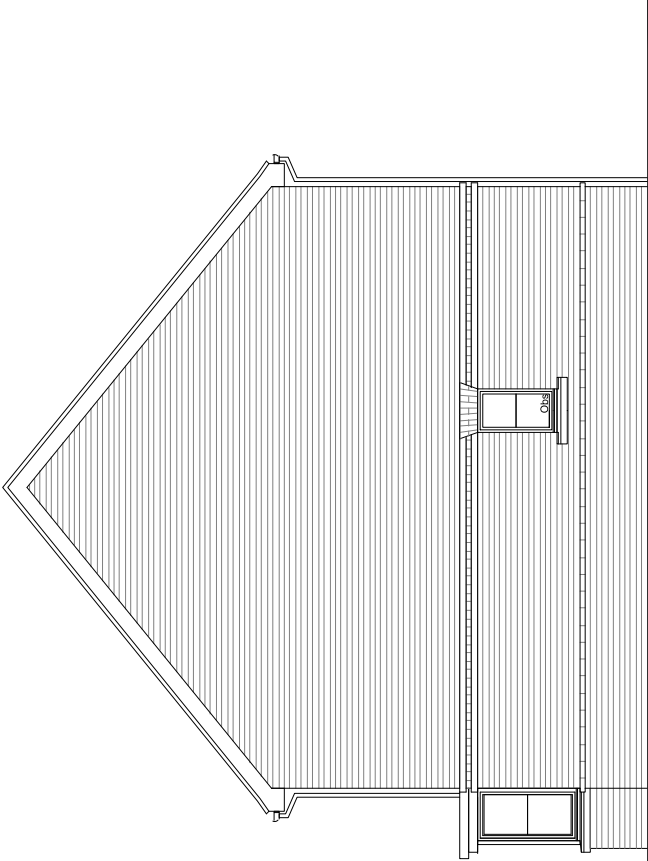
Side Elevation Obs - Obscured Glazing
