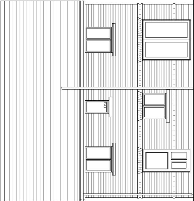
Rear Elevation Obs - Obscured Glazing
