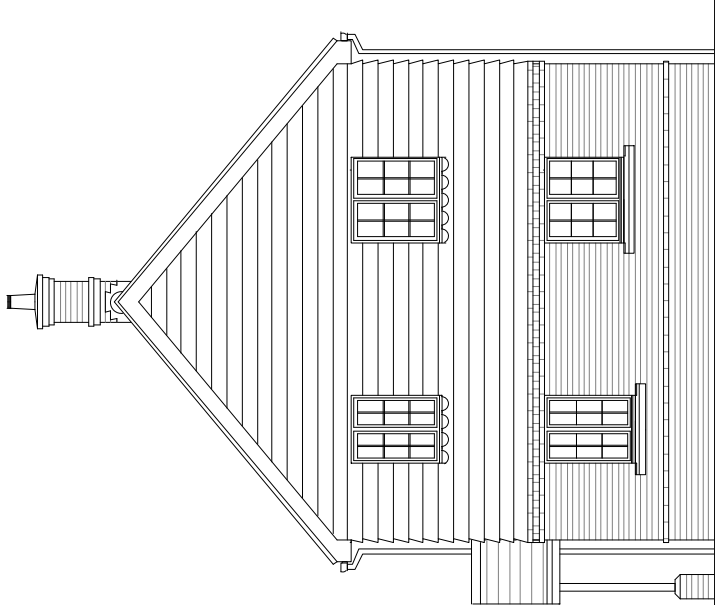
Side Elevation Obs - Obscured Glazing
