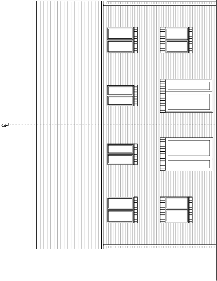
Rear Elevation
