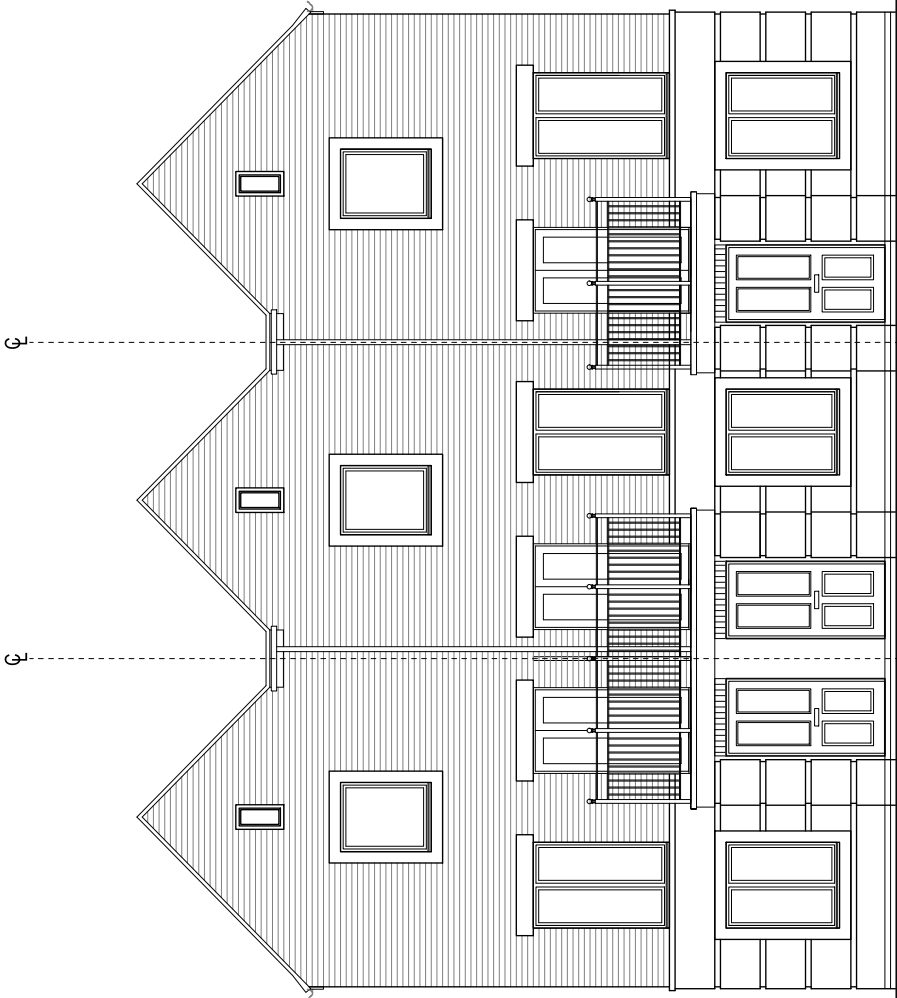
Front Elevation
