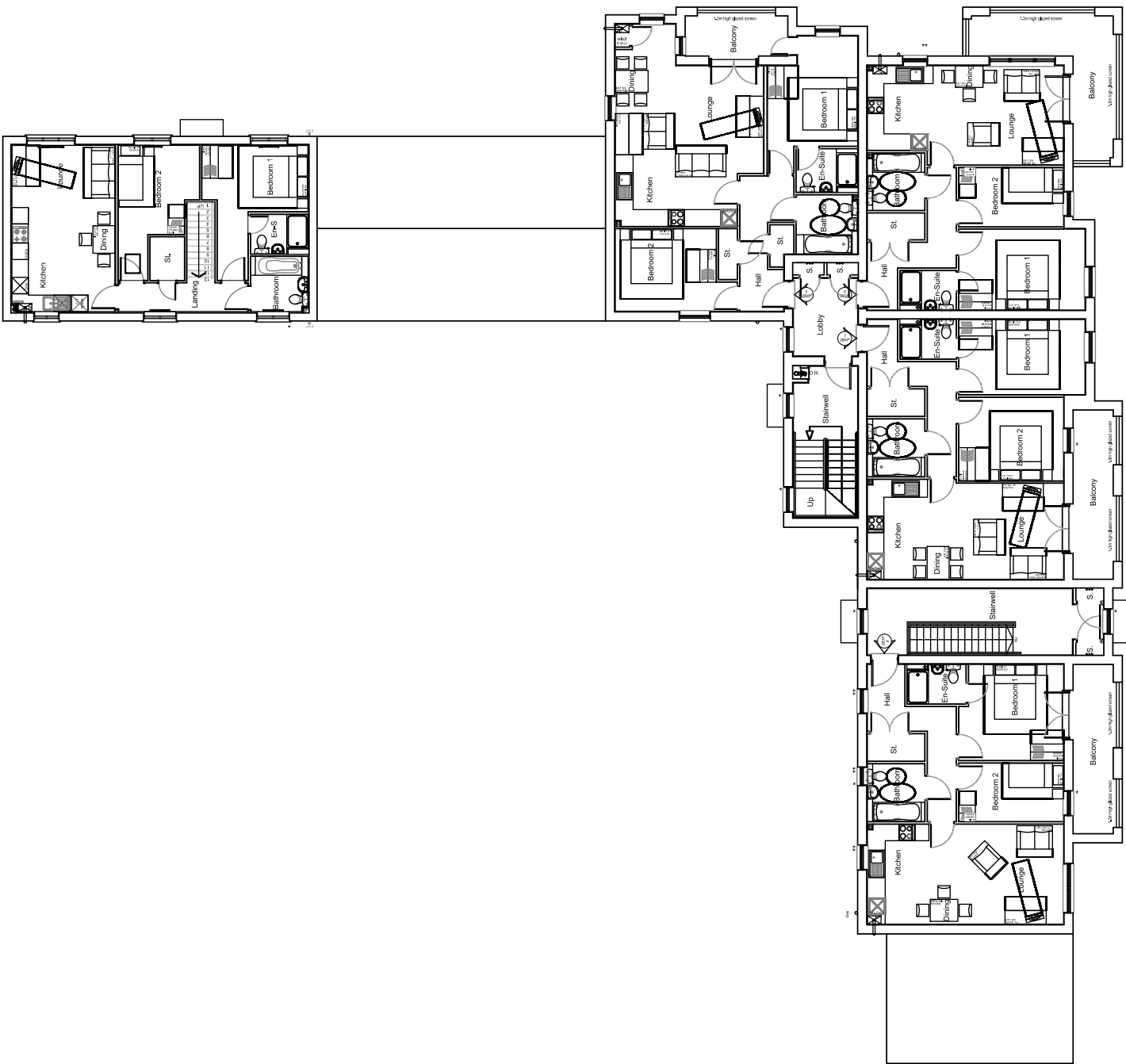
First Floor Plan ** - False Panel * - Obscured Glazing
