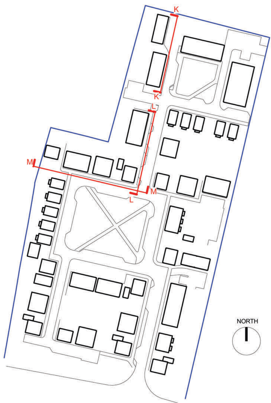
KEY PLAN
