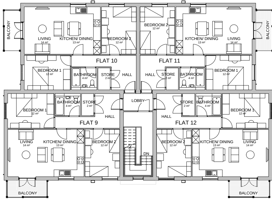
SECOND FLOOR PLAN 1 : 100
